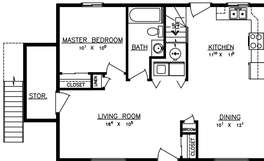
MAIN FLOOR AREA = 768 S.F.
